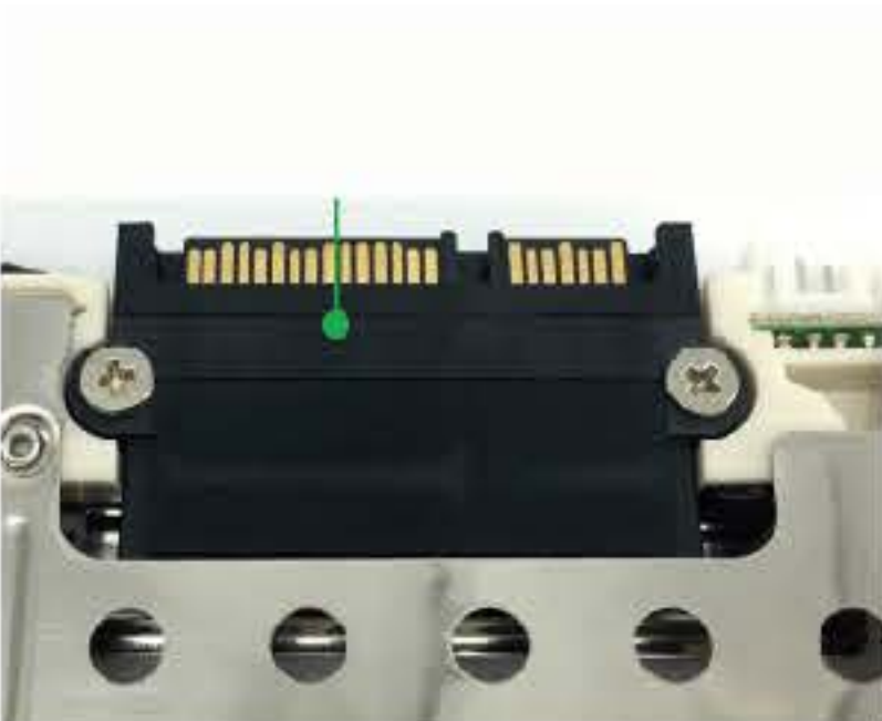
Non-scratch SATA connector (NSS) allows Hard Drive hot-swap life cycle for more than 50,000 duty cycles.
